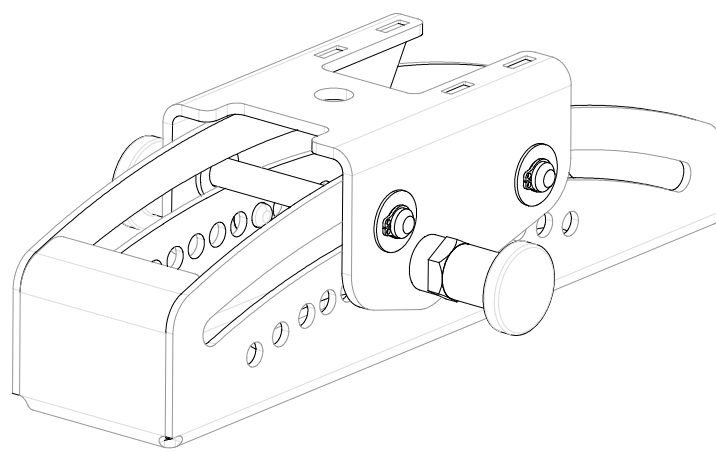
ASSEMBLED VIEW
