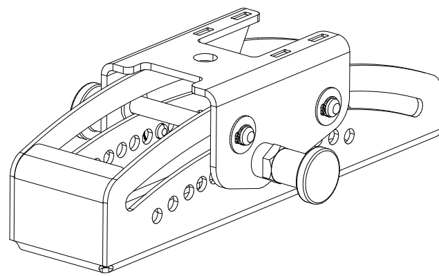
ASSEMBLED VIEW
